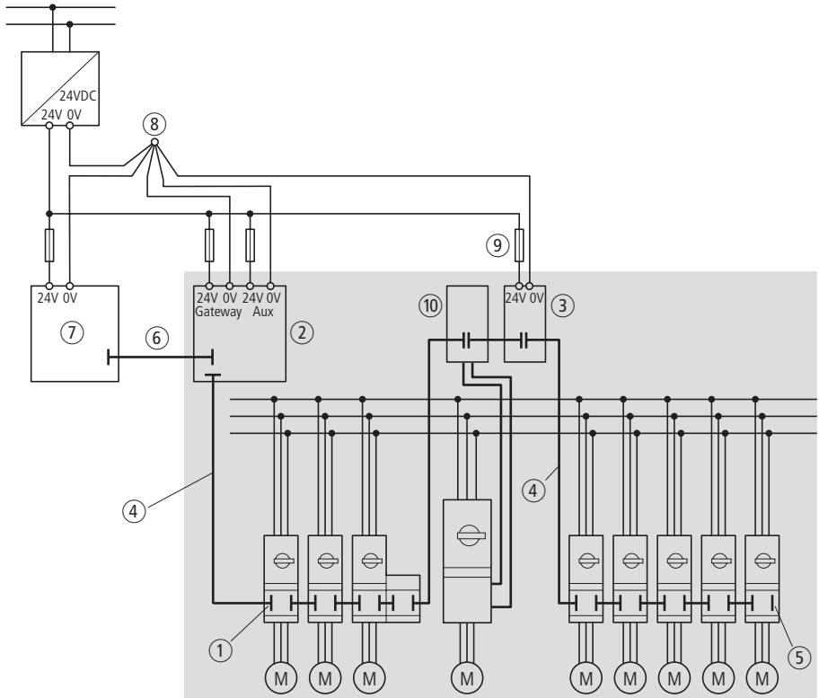
Figure 1: Assembly, connection system SmartWire
