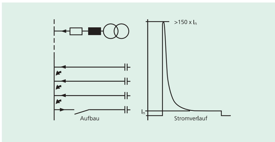
Bild 10: Special Type DIL K capacitor switching contactors can be used to switch banks of capacitors for power factor compensation purposes. The charging resistors reduce the extremely high inrush current peaks. Regular DILM contactors can be used for individual compensation or when capacitor banks are equipped with inductive choking means.
